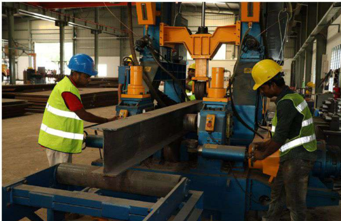
H-Beam Fabrication
